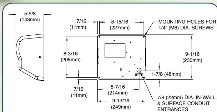
Figure 1 - EXT Series Surface Mount
